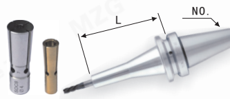
SDC Back-Pull Collet Toolholder
